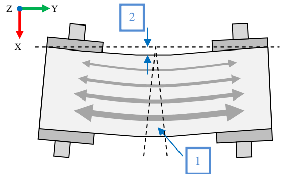
Figure 3: Conventional steering mechanisms introduces both stretch of the belt [1] and deflection in the printing area [2]
