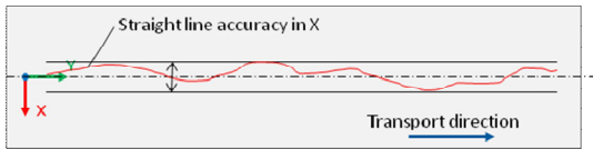
Figure 5: Definition of straight-line accuracy
